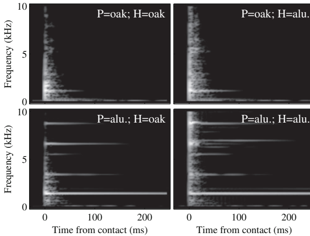
Fig. 4.2 Detail of the spectrotemporal structure of impact sounds generated by striking a 450\text{ cm}^2 square plates (P) made of oak or aluminium with an aluminium or oak hammer (H). Level from low ( black ) to high ( white ). Data from Giordano et al. (2010)
